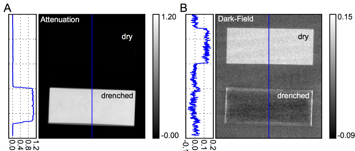
Fig 2. Complementarity of X-ray attenuation and dark-field radiography. X-ray attenuation (A) and dark-field (B) signal of dry (upper) and water drenched (lower) open cell melamine sponges. Similar to the human lung, a fine-pored melamine sponge comprises thousands of air-tissue interfaces and causes strong ultra small-angle X-ray scattering and therefore exhibits a distinct dark-field signal. At the same time, comprising porous structures, both lung and sponge yield small overall densities and appear radiolucent in the attenuation channel. When drenching the foam, air is displaced by water resulting in a high contrast in the attenuation channel due to stronger attenuation in comparison to air. Simultaneously, the interfaces become neutralized, explaining an inversion of both contrast modalities. The image acquisition protocol except for the tube current was similar to the one of the dead body scan (70 kVp, 100mA, 20 ms exposure time per pulse, 12 Hz pulse frequency, 3x3 pixel binning).
