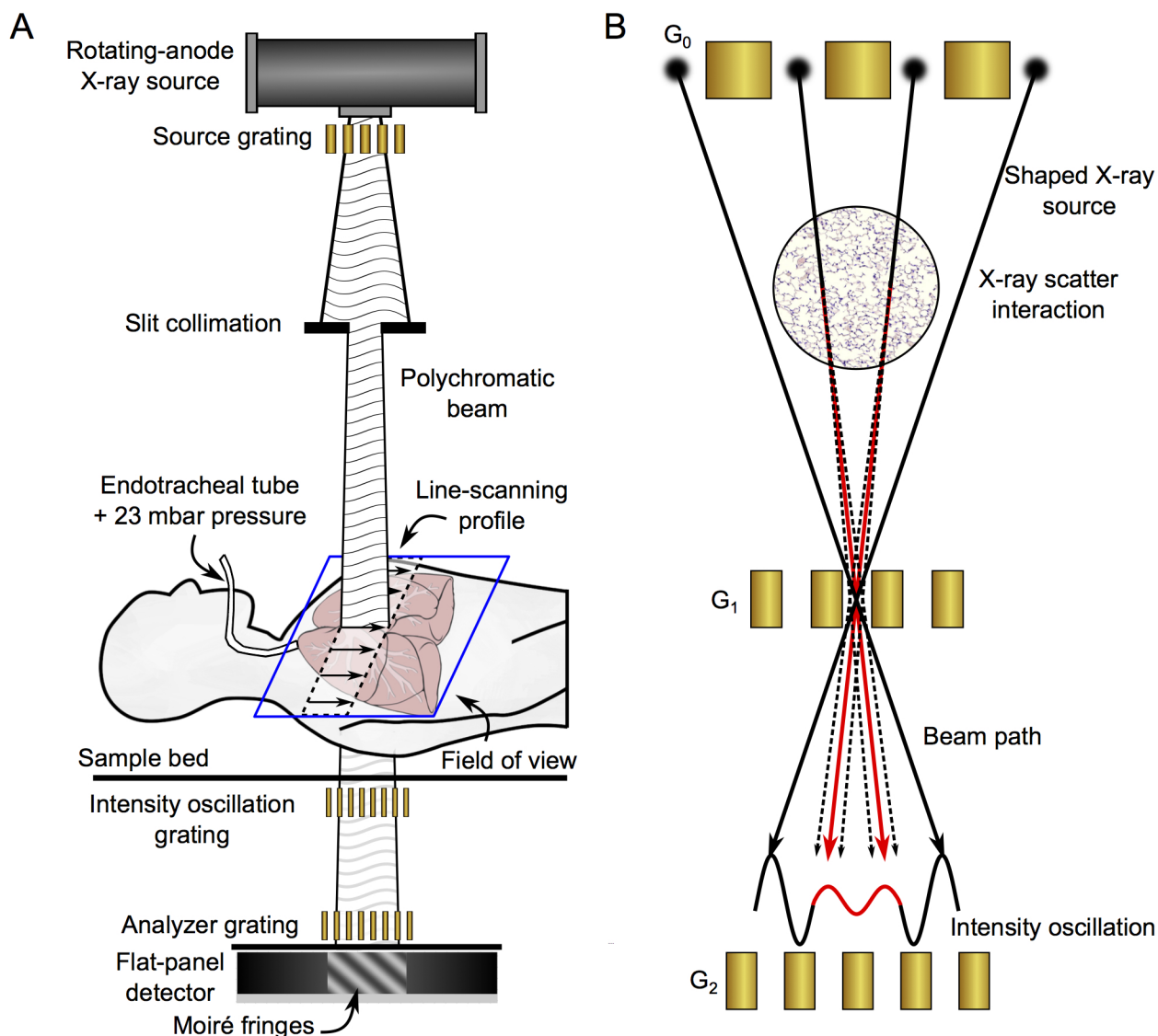
Fig 1. Human X-ray dark-field prototype chest scanner. (A) The X-ray chest scanner combines a three-grating arrangement (with an oblong active area) with a continuous line-scanning approach, with the purpose of imaging an entire human thorax. By scanning the active area over the field of view, every pixel is sampled at various phases of the Moiré pattern, allowing retrieval of attenuation, differential-phase, and dark-field information. In order to simulate in-vivo conditions and demonstrate clinical relevance of the presented results, tracheal intubation was performed on the deceased body and the lungs were inflated at 23 mbar during measurement. (B) X-ray dark-field contrast is generated by ultra small-angle scattering for instance at air-tissue interfaces of lung alveoli. Scattering causes blurring (red) of the initially well-delimited (black) intensity pattern generated by G 1 resulting in a reduction of the measured visibility. Note that several slit sources contribute to the intensity value at any specific location in front of G 2 . For sake of simplicity, only a few rays passing through one G 1 slot are shown for illustrational purposes.
